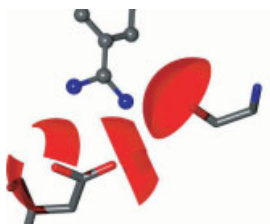
Fig. 7.3 Interaction surfaces of three hydrogen bond acceptors in thrombin (shown in red). Protein atoms are drawn with sticks, ligand atoms with balls &
