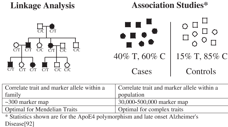
Fig. 3.1 Strategies for genetic analysis.
